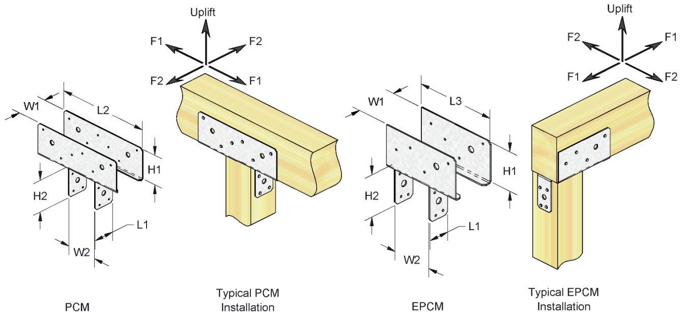
FIGURE 8—PCM AND EPCM POST CAPS
