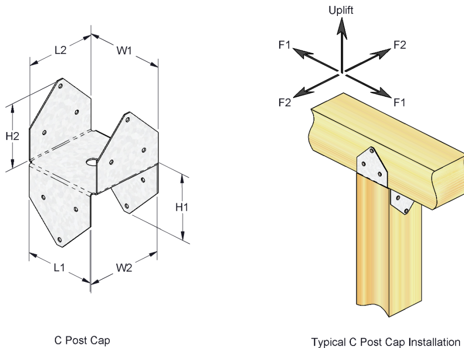
FIGURE 1—C POST CAP
